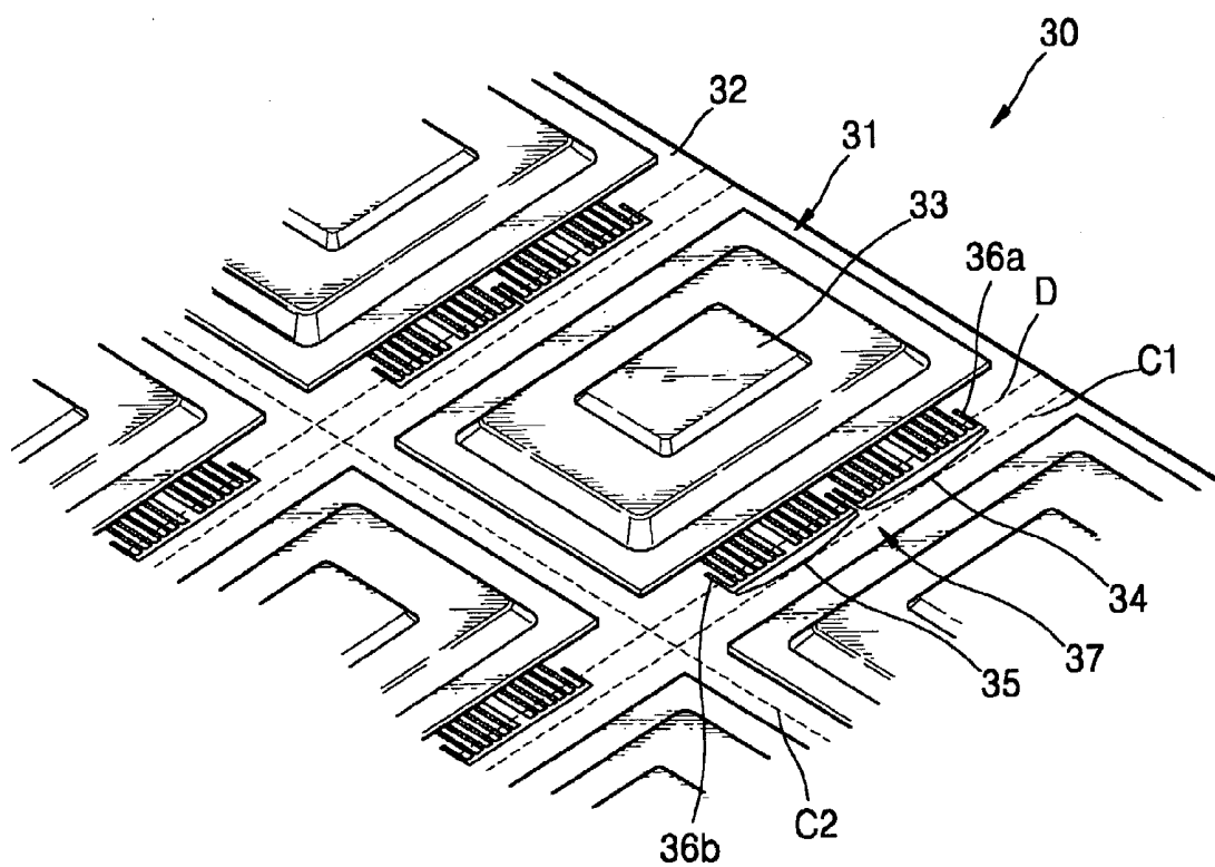
FIG. 3 (PRIOR ART)
